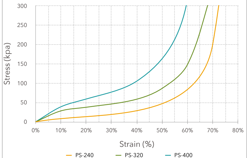
PS series CFD Curve
